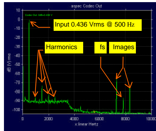
Figure 3 - Distortion, Noise and Images
