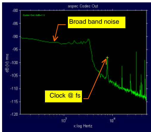
Figure 2 - Output Noise Spectrum of EVM
