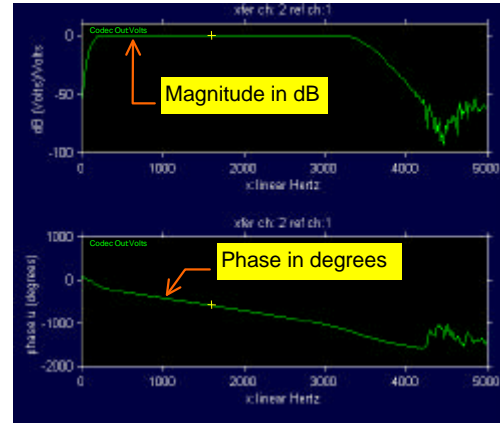
Figure 6 – Codec Frequency and Phase Response
