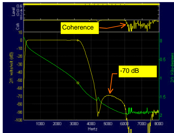
Figure 8 – Swept-sine Transfer Function Measurement
