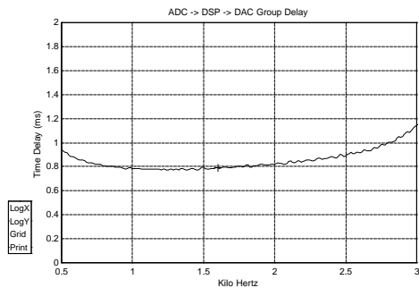
Figure 7 – Group Delay in Milli-seconds
