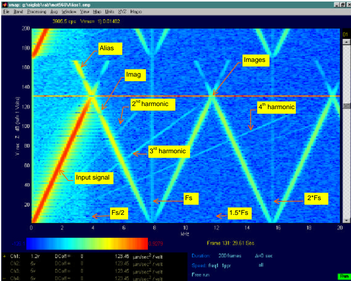
Figure 9 – Spectral Map Display of Analog I/O Subsystem Showing Noise ( f < 3000 Hz), Harmonics, Images, Aliases, and Sampling Clock Feedthrough.
