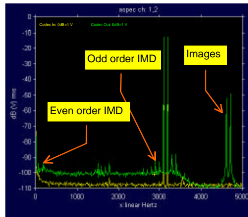
Figure 4 - Intermodulation Distortion, and Images
