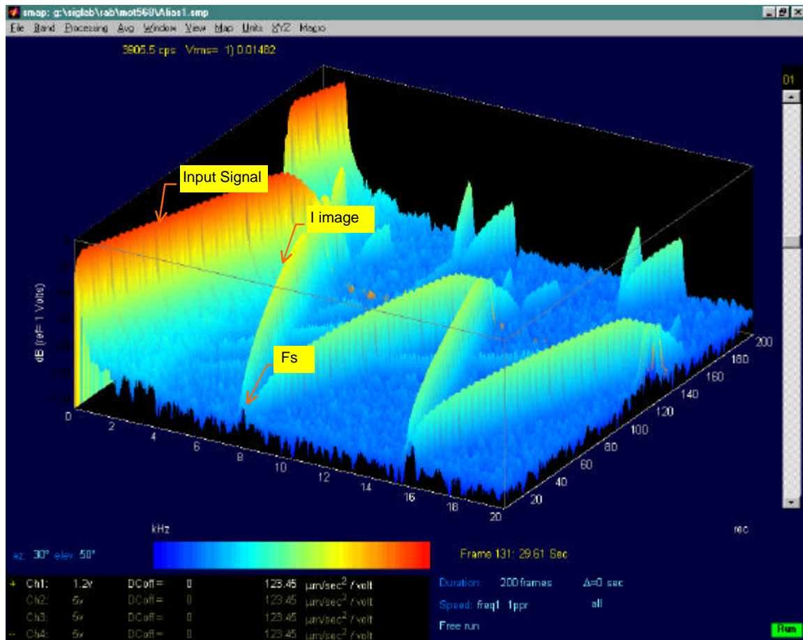
Figure 10 – “Waterfall” Display of Analog I/O Subsystem Showing Noise ( f < 3000 Hz), Harmonics, Images, Aliases, and Sampling Clock Feedthrough.
