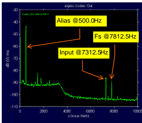
Figure 5 - Alias at 7812.5-7312.5=500 Hz
