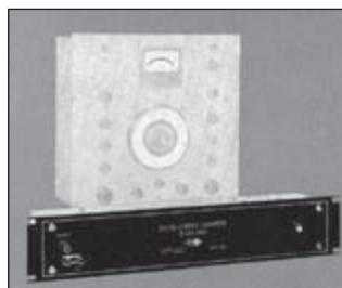
Figure 3. Model SD 11, COLA Constant Output Level Adapter with a Brüel & Kjær vibration exciter controller in the background.
