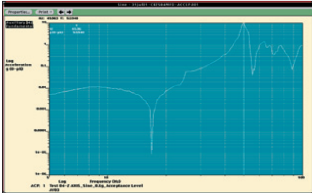
Figure 53. Same data as previous but showing tracking filtered fundamental response.
