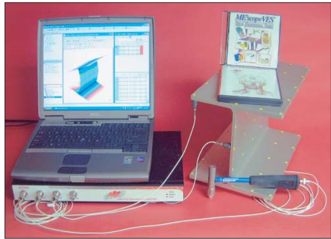
ME'ScopeVES uses Vibration Research 8500 shaker-controller to acquire impact data.
